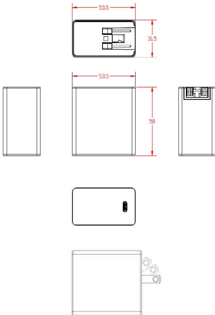
TMW65CU standard model with embedded foldable US AC plug
